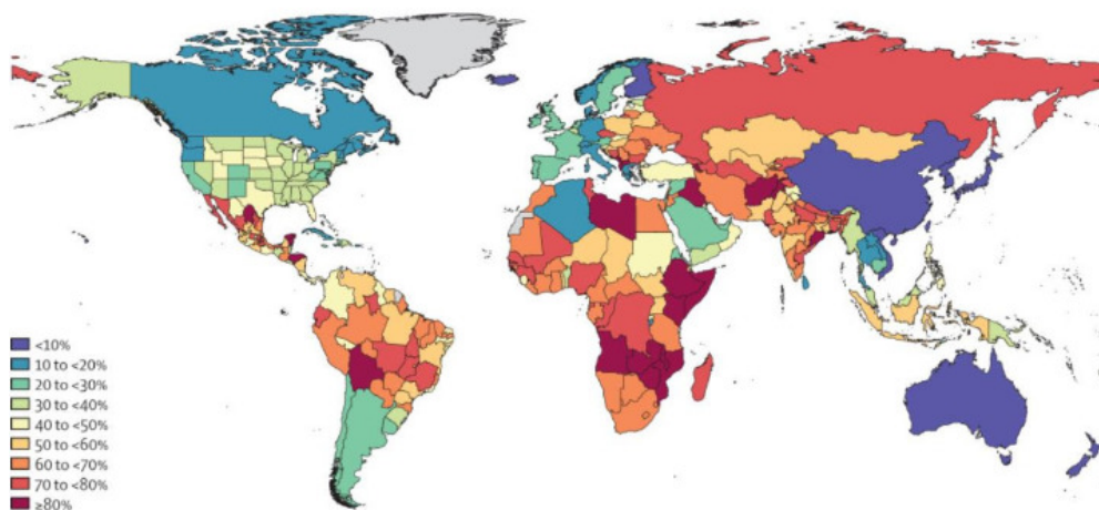
Figure 3 Cumulative proportion of the population infected with SARS-CoV-2 at least once by Nov 14, 2021, by country and territory
